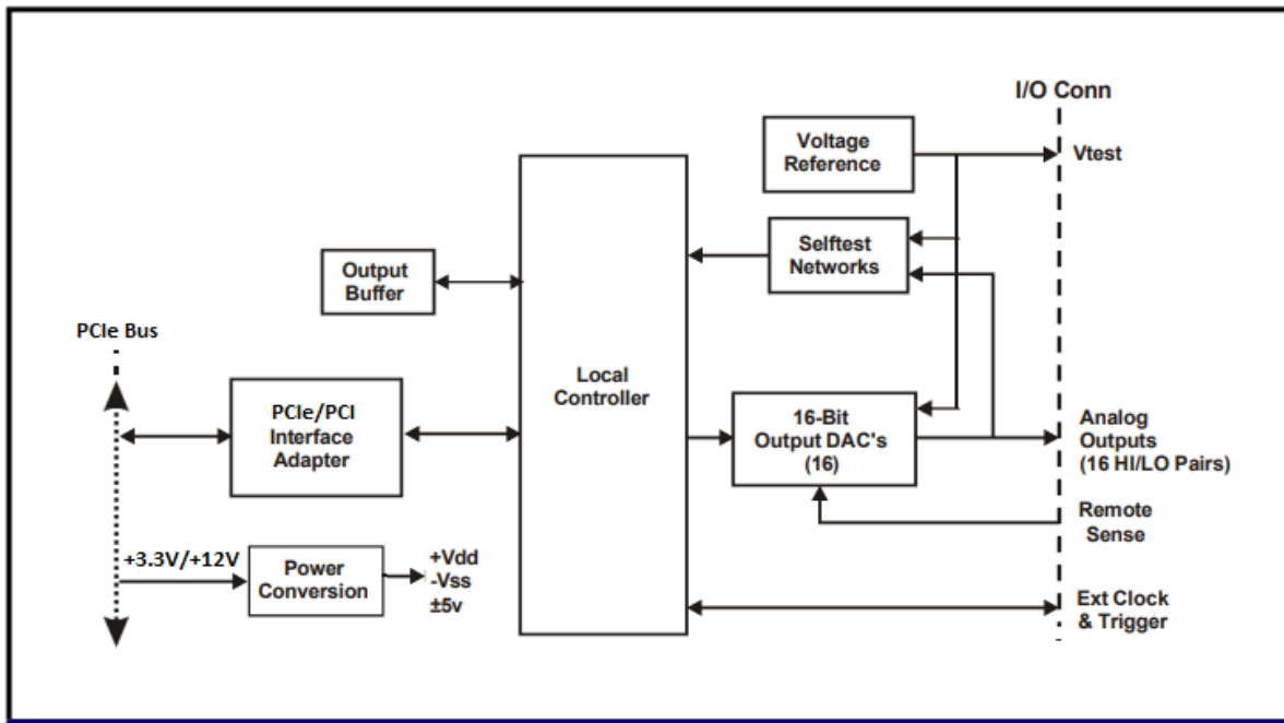
Figure 1.2-1. Functional Organization
