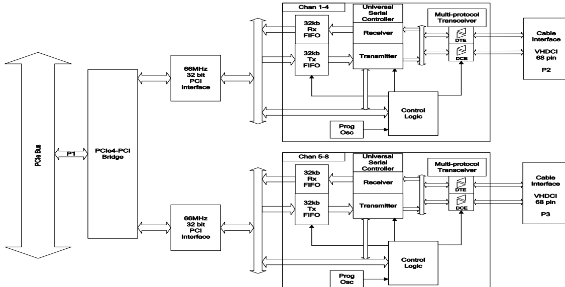
Figure 1-1 Block Diagram of PCIe4-SIO8BX2V-SYNC
