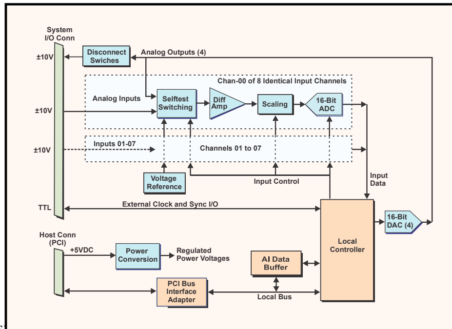
Figure 1. PMC66-ADADIO2 Analog I/O Board, Simplified Functional Diagram
